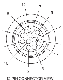
Wiring Diagram ( Connector Option E )
