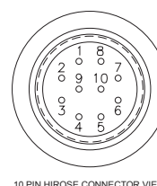
Wiring Diagram ( Connector Option H )
